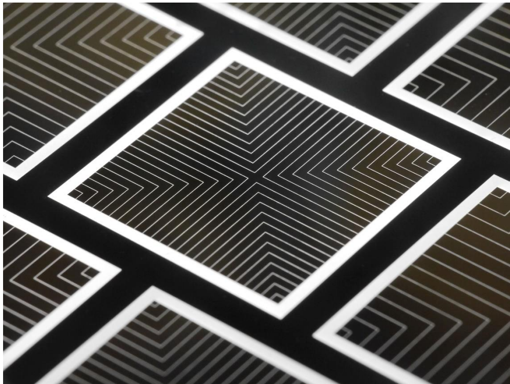
The TOPCoRE solar cell achieved 26 percent efficiency, a new world record for both-sides-contacted solar cells. ©Fraunhofer ISE
